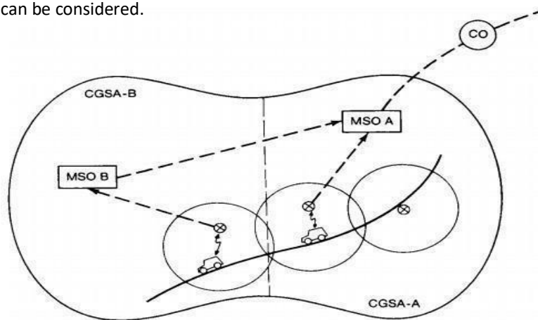
Fig.7. Intersystem handoffs
