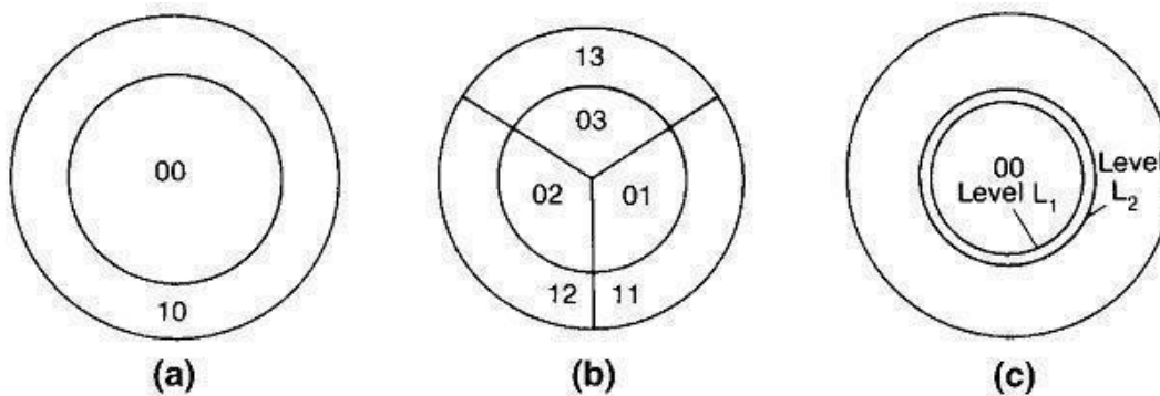
Fig.4.5. Under laid-overlaid cell arrangements. (a) Underlay-overlay in omniscell; (b) Underlay-overlay in Sectorized cell; (c) Two level handoff scheme
