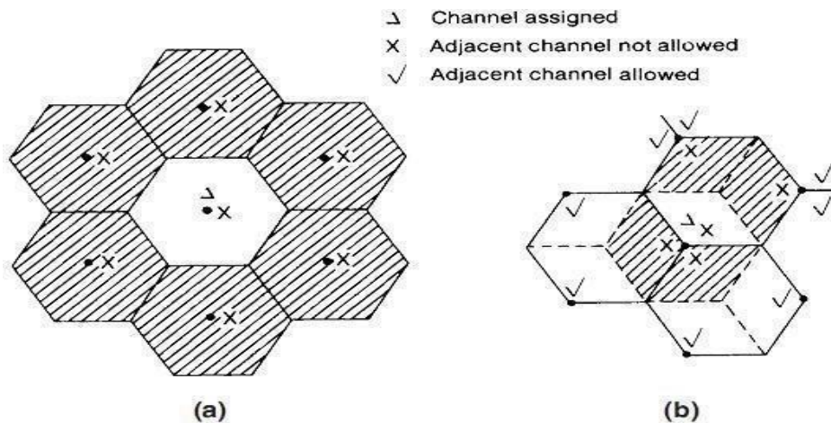
Fig.4.3 Adjacent channel assignment (a) Omni direction antenna cells; (b) Directional antenna cells
