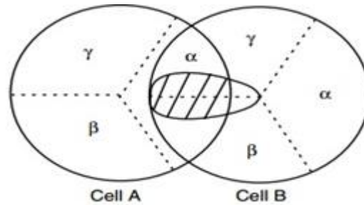
Fig 10.3 Soft-Softer Handoff
