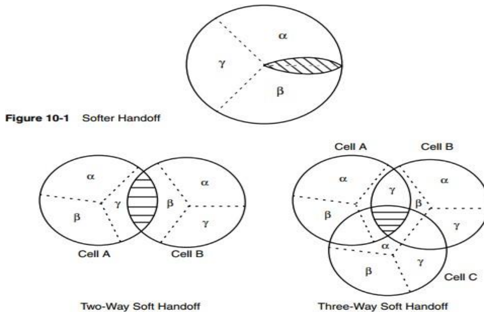
Figure 10-2 Soft Handoff
